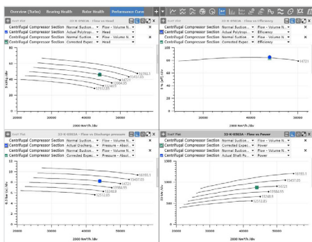
System 1 compressor performance plots
