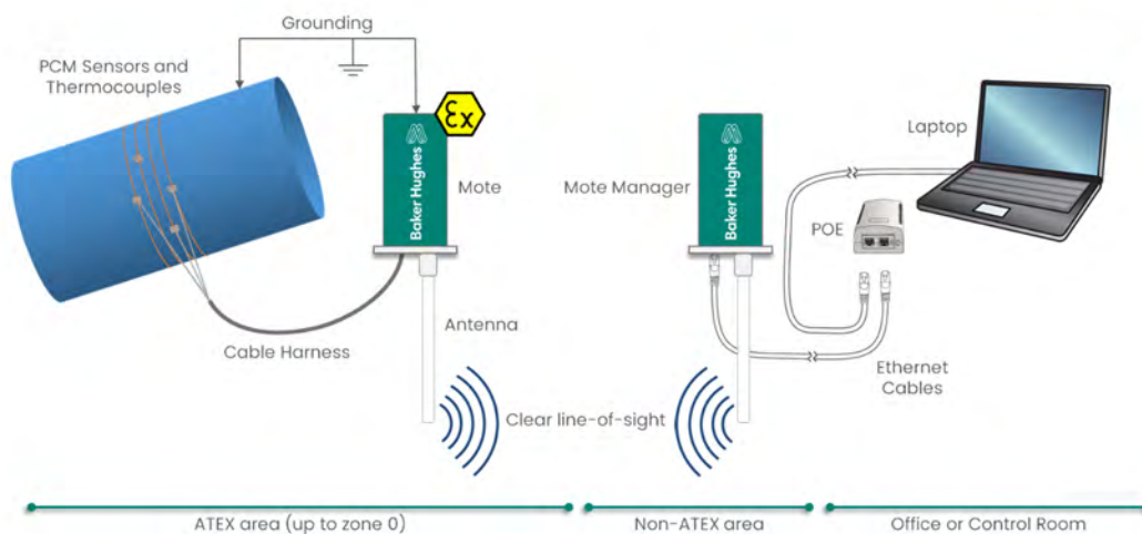
Figure: Schematic representation of the PCM system
