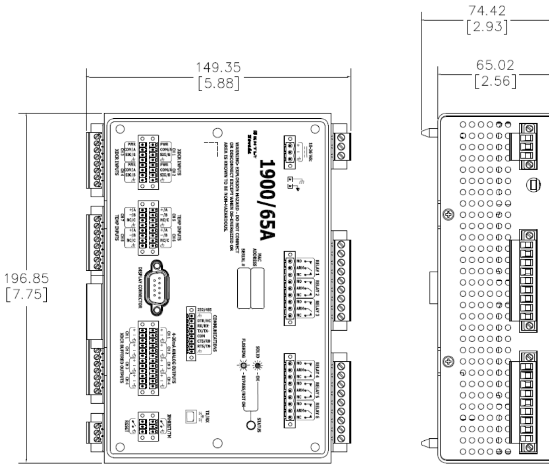
Figure 1: Monitor Module Dimensions
