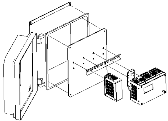
Figure 4: 1900/55 Replacement Kit
